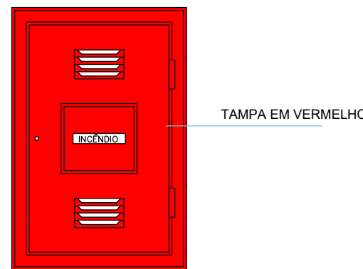
VISTA FRONTAL
